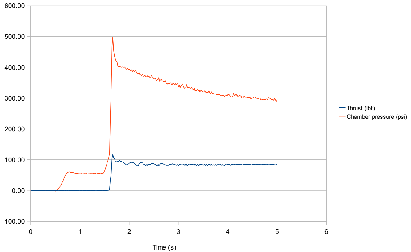
Tropos 2 Corn Syrup/Sugar Static Firing First 5 seconds, 20 April 09
